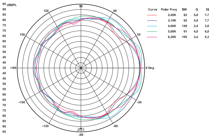
SPL vs Angle
