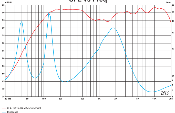
SPL vs Freq
