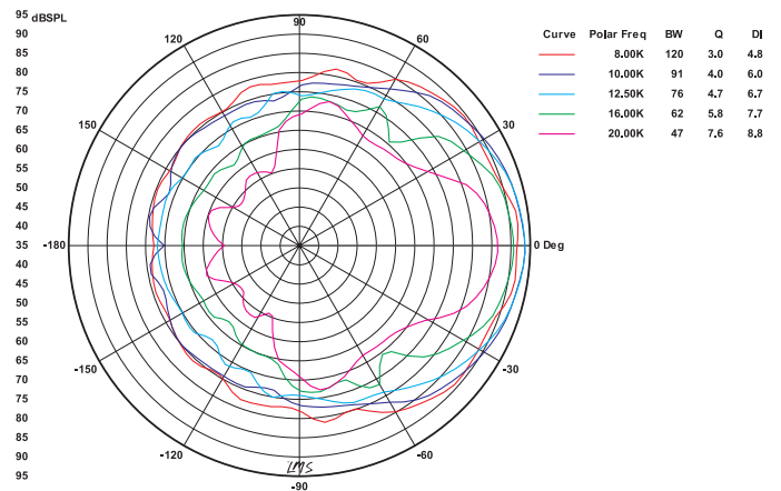
SPL vs Angle
